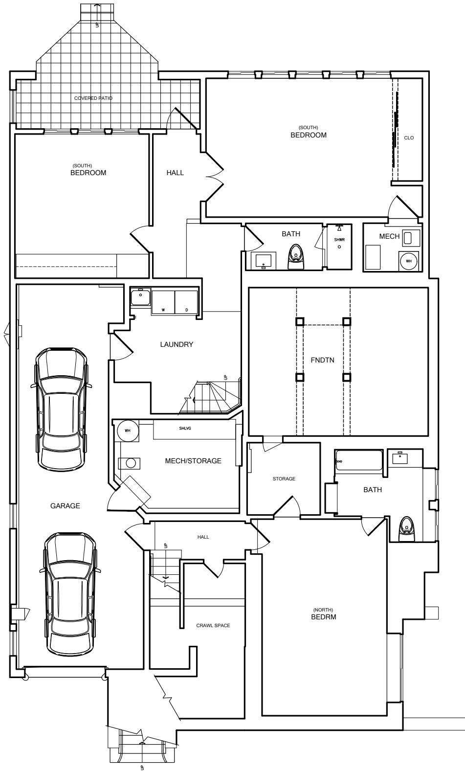
EXISTING BASEMENT LEVEL FLOOR PLAN
