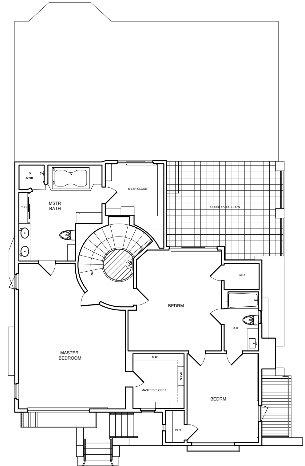
EXISTING SECOND LEVEL FLOOR PLAN
